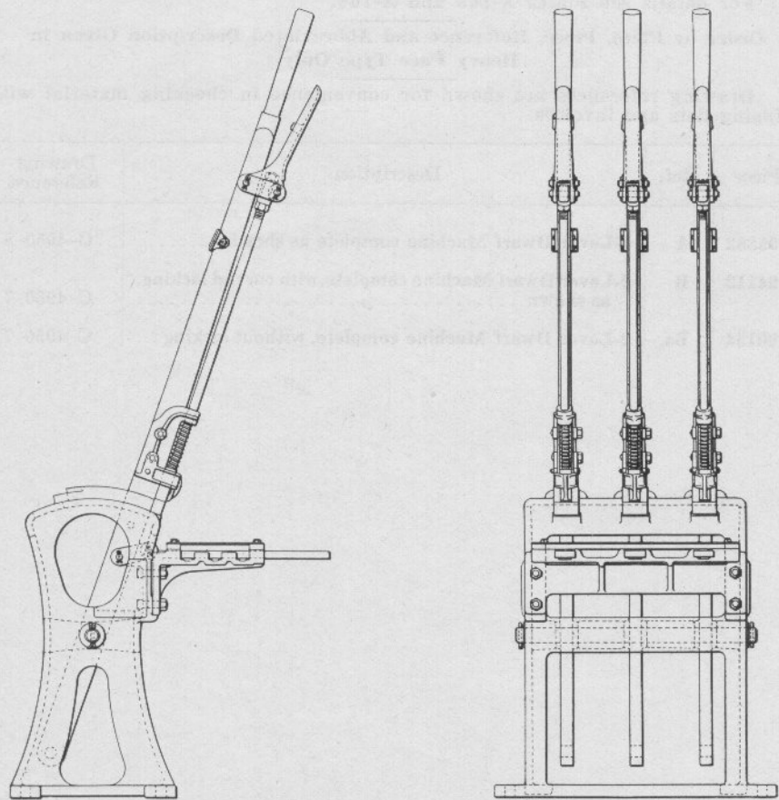
THE DWARF INTERLOCKING MACHINE ARRANGED FOR CONNECTIONS ABOVE FLOOR
